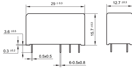
5mm Pinning (HF115FD/ □□□ -□□ -2/3-□)
